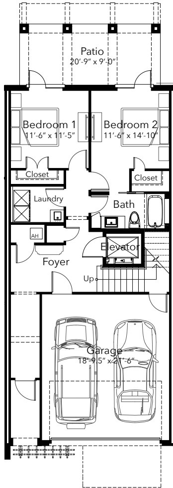
1 st Floor
