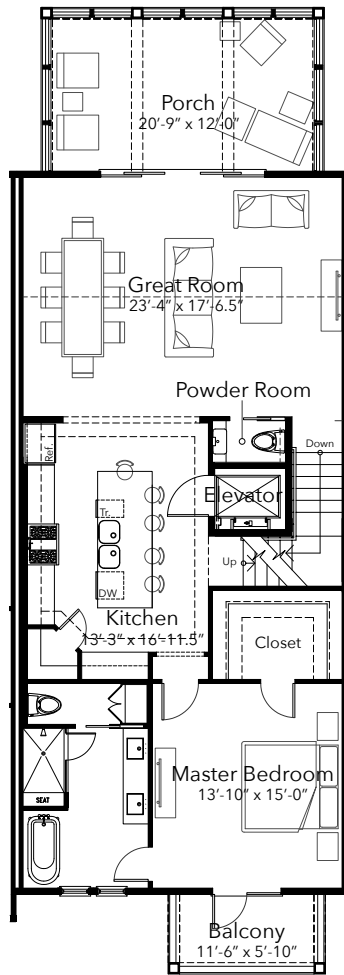
2 nd Floor
